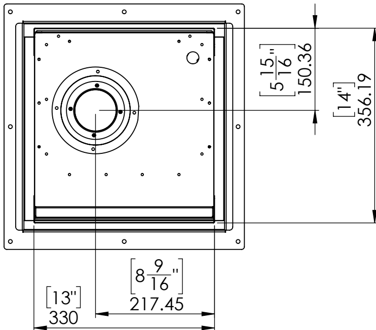
Back View
