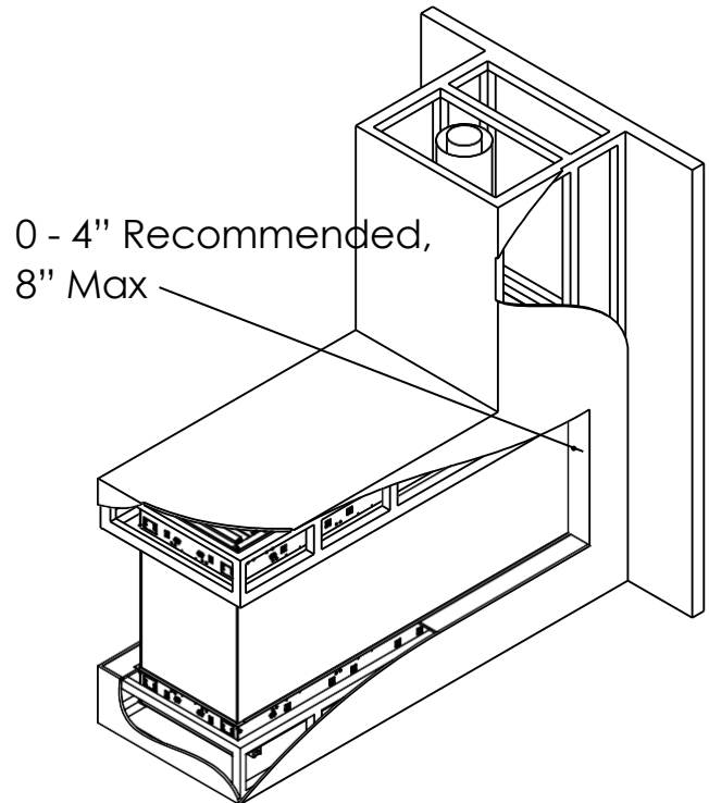
Recessed Installation
