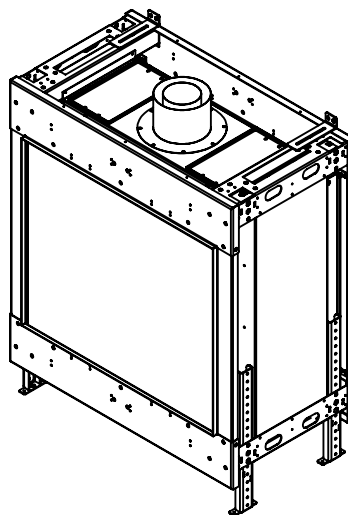
Telescopic Leg Range From bottom of glass: 10"-19"
